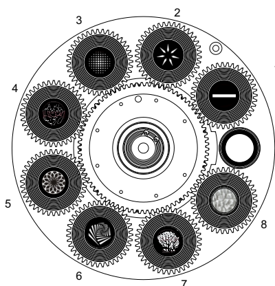
Rotierendes Goborad/ rotating gobo wheel
