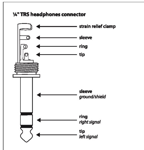
Fig. 5.6 Headphones stereo plug
