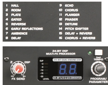
Fig. 4.20 Multi-effect processor
