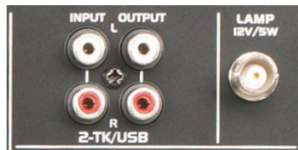
Fig. 4.15 RCA connectors and lamp socket
