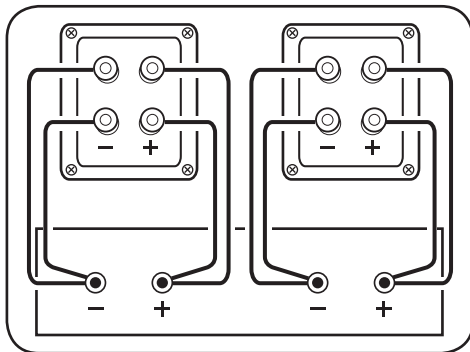
Bi-Wiring
