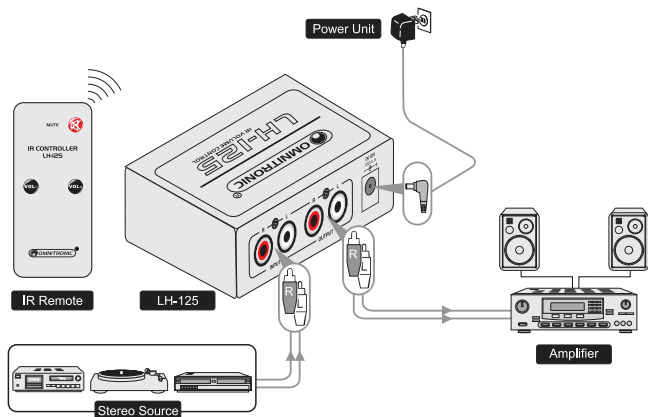
Fig. 4-1 Connection Example
