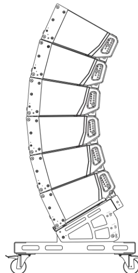
6 pcs curved
