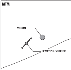
1-V, 3 WAY LEVER SWITCH
