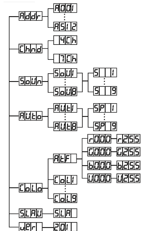
Menu structure
